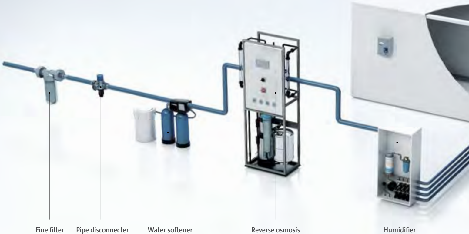
Schematic diagram of a water treatment system for adiabatic humidification
